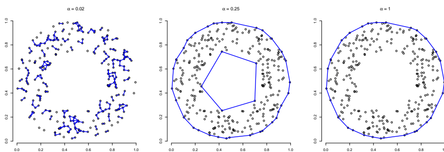
Figure 3: Influence of the parameter \alpha on the \alpha -shape. From left to right, \alpha -shape of a random sample of size n = 300 on the annulus with outer radius 0.5 and inner radius 0.25 for \alpha = 0.02, 0.25, 1 .
