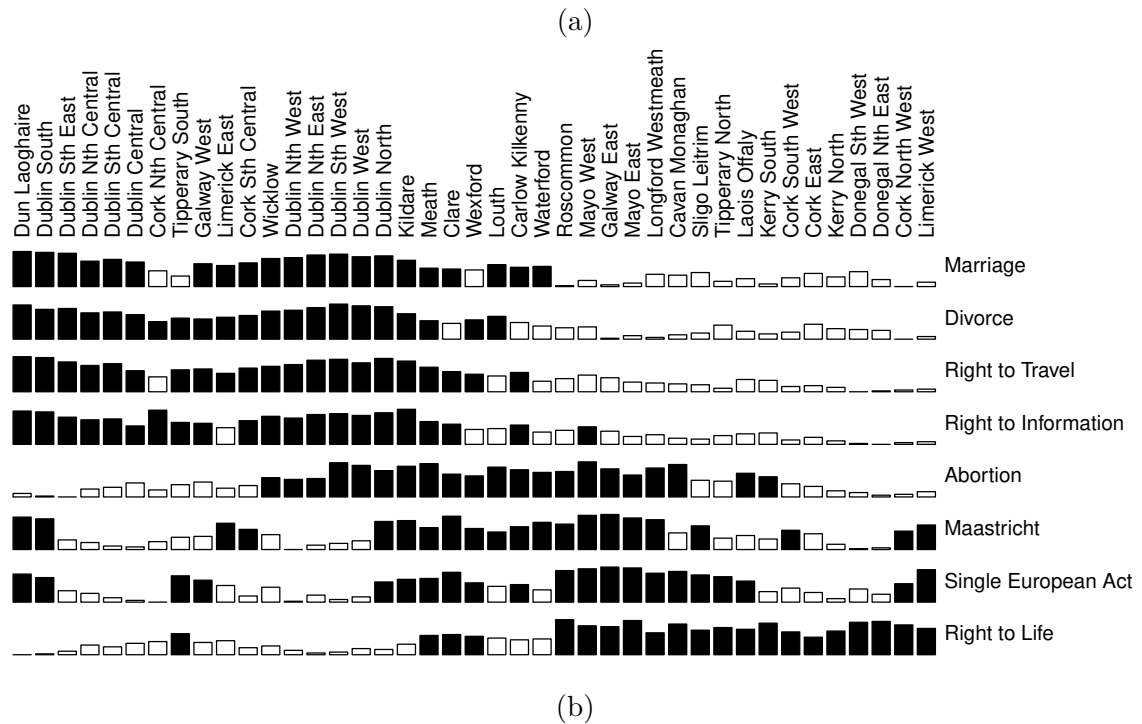
Figure 7: Bertin plot for the (a) original arrangement and the (b) reordered Irish data set.
